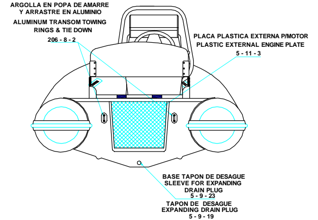
AFT VIEW VISTA TRASERA
